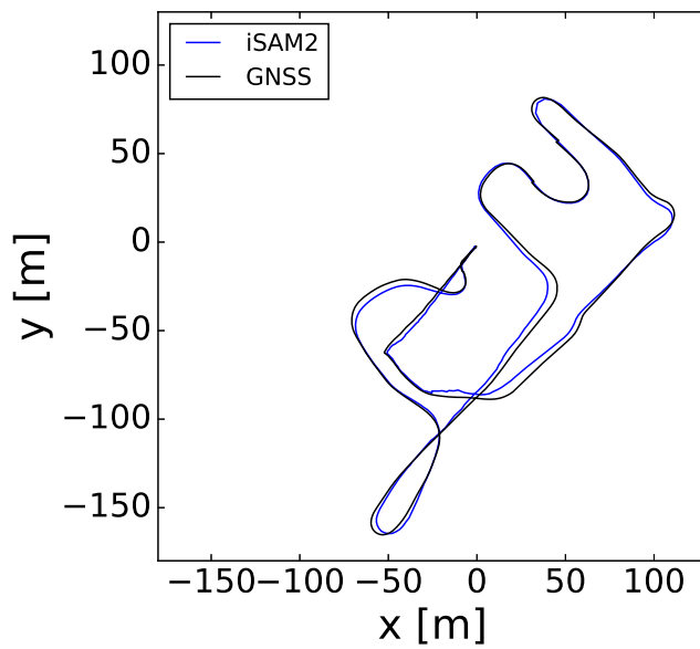
Figure 7.22 Trajectory when loop closure is implemented with the odometry and IMU is fused into the system.
