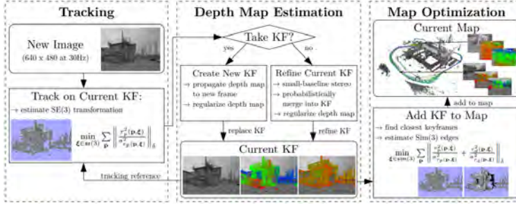
Figure 3.2 Overview over the complete LSD-SLAM algorithm. Image and caption taken from [10].
