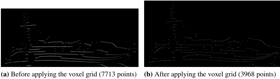
Figure 6.6 Lidar data before and after applying the voxel grid filter.
