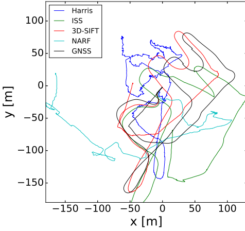
Fig. 6. Trajectory of different keypoint extractors
