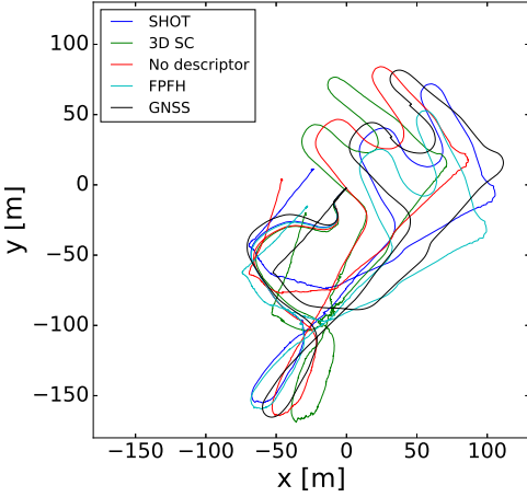
Fig. 10. Trajectory of SIFT using different keypoint descriptors
