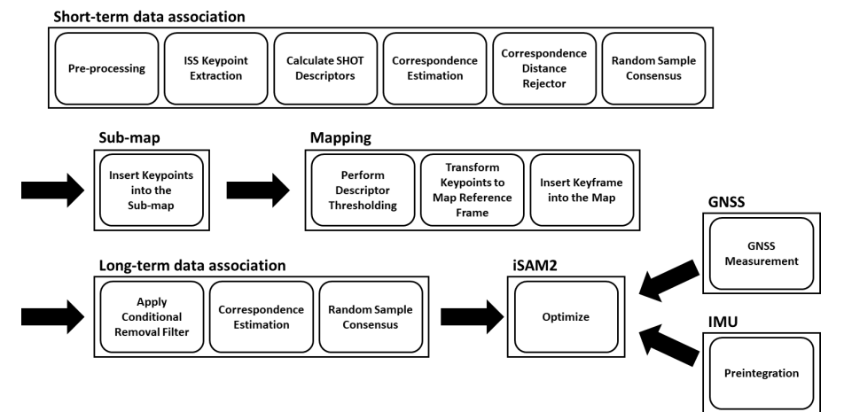
Figure 6.2 SLAM system pipeline.
