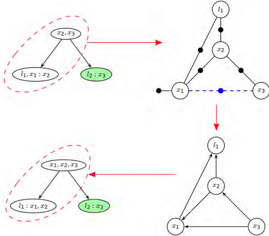
Figure 3.4 Updating a Bayes tree with a new factor, based on the example in Fig. 3.3c. The affected part of the Bayes tree is highlighted for the case of adding a new factor between x_1 and x_3 . Note that the right branch is not affected by the change. (top right) The factor graph generated from the affected part of the Bayes tree with the new factor (dashed blue) inserted. (bottom right) The chordal Bayes net resulting from eliminating the factor graph. (bottom left) The Bayes tree created from the chordal Bayes net, with the unmodified right “orphan” sub-tree from the original Bayes tree added back in. Image and caption taken from [11].
